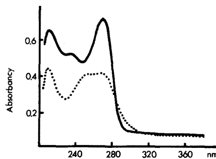
Fig.5. Ultraviolet absorption spectra of the coupling products of PITC and Ala (dotted) which resulted in PTC-Ala, and PITC and NMA 1 (solid) which resulted in PTH-NMA 1 . The coupling solution is 67% aqueous pyridine.
